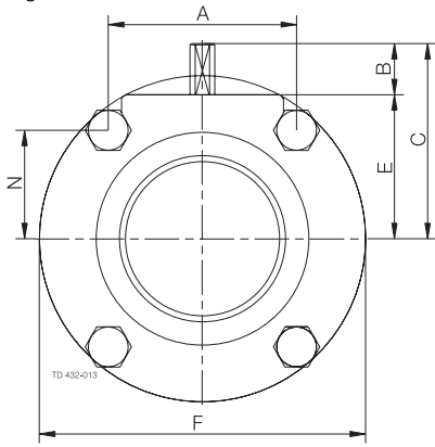
Fig. 1. Dimensions - valve.
