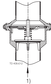
Fig.3 1 = Flow direction.
